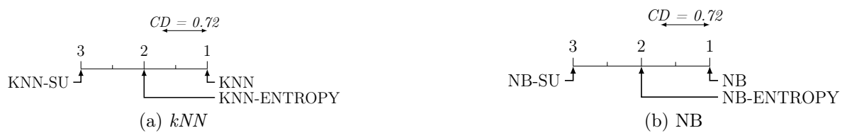
Figure 7.4: Critical differences chart for the processing time (CPU Time) obtained by weighted classifiers.
