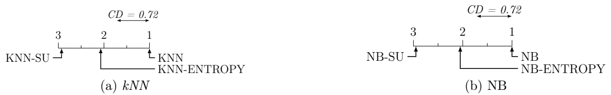
Figure 7.5: Critical differences chart for the memory consumption (RAM-Hours) obtained by weighted classifiers.
